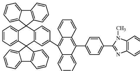
Chemical Compound 208
