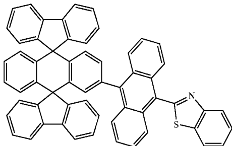
Chemical Compound 214
