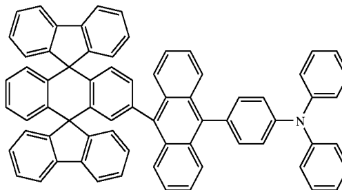
Chemical Compound 401
