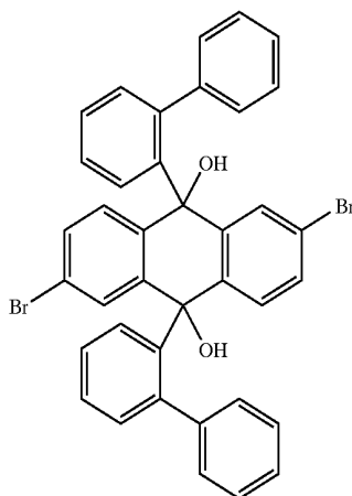
2,6-dibromo-9,10-bis(2-biphenyl-dihydroxy)-anthracene
