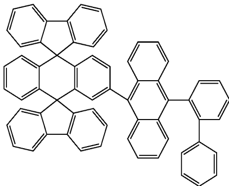
Chemical Compound 111
