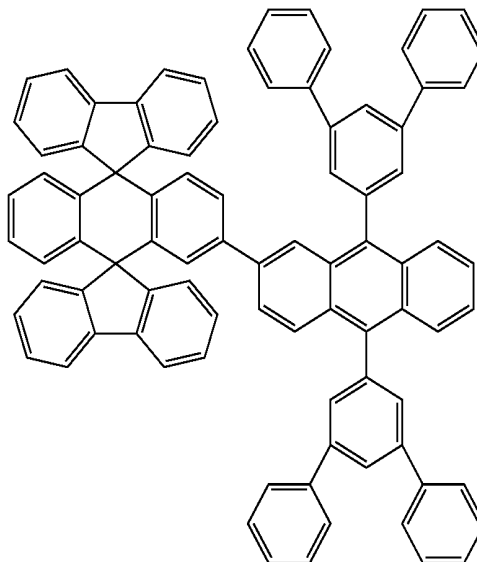
Chemical Compound 119
