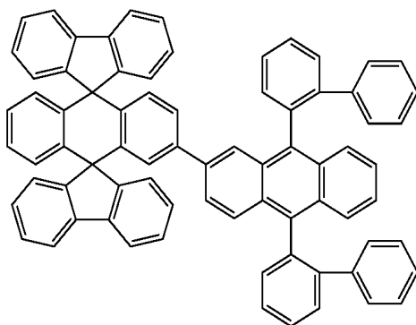
Chemical Compound 118
