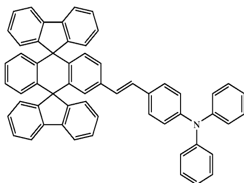
Chemical Compound 400
