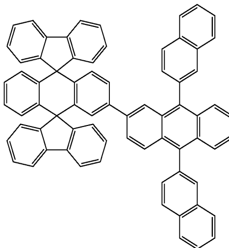
Chemical Compound 117
