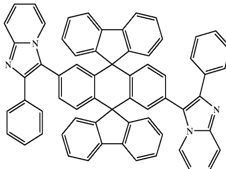
Chemical Compound 413
