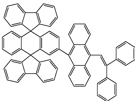
Chemical Compound 137
