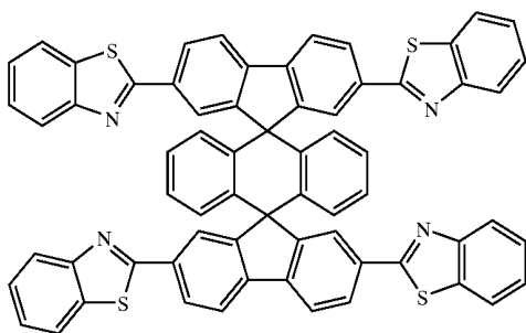
Chemical Compound 218
