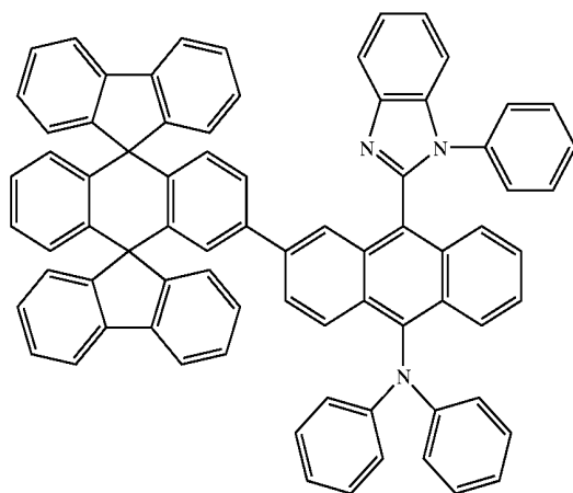
Chemical Compound 127
