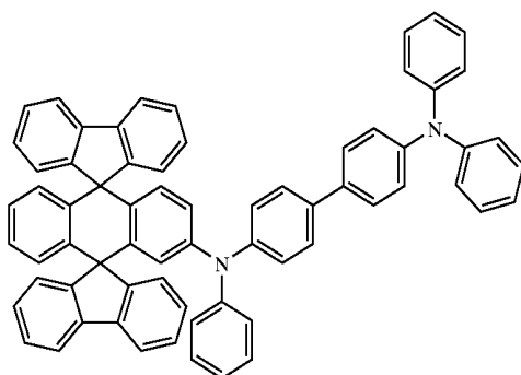
Chemical Compound 307
