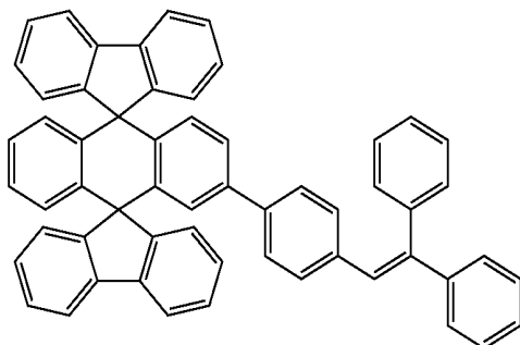
Chemical Compound 107
