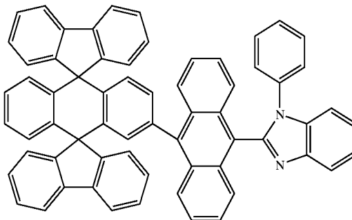
Chemical Compound 200
