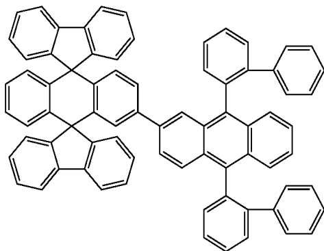
Chemical Compound 118
