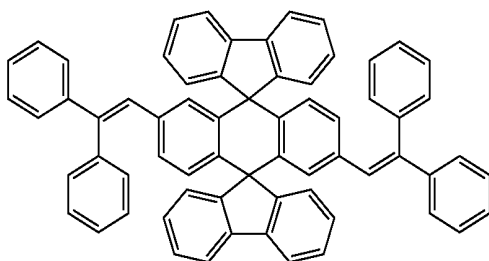
Chemical Compound 105
