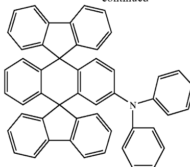
Chemical Compound 11
