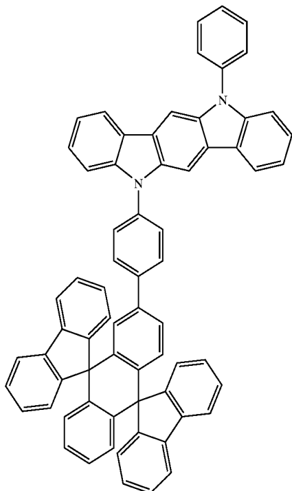
Chemical Compound 412
