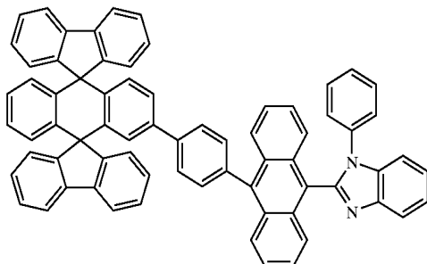
Chemical Compound 207
