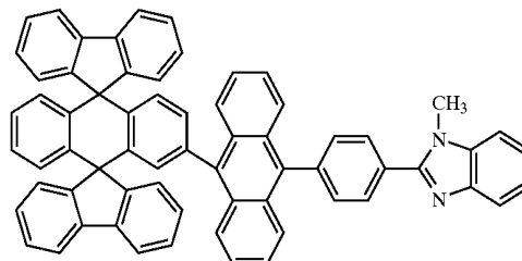
Chemical Compound 208
