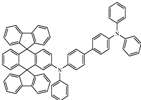
Chemical Compound 307
